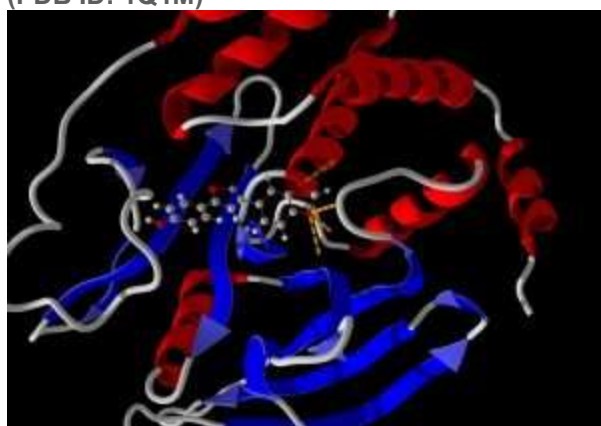
FIG. 3: DOCKING POSE OF COMPOUND IIE WITH RECEPTOR PTP1B RECEPTOR (PDB ID: 1Q1M)
